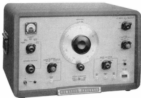
Fig. 1. New -hp- Model 686A voltage-tuned sweep oscillator provides c-w, f-m, a-m and swept outputs over 8.2 - 12.4 kmc range. Sweep widths as wide as full band can be selected at a wide range of rates to suit measurement conditions.
