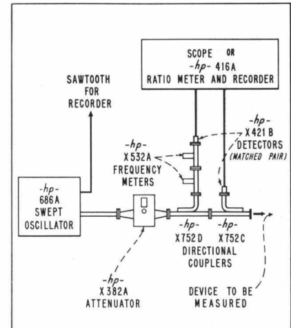
Fig. 4. Equipment arrangement for measuring reflection coefficient magnitude in either permanent form or as viewed on meter or oscilloscope trace. Wavemeters in incident arms are used to insert marker pips at desired points.
